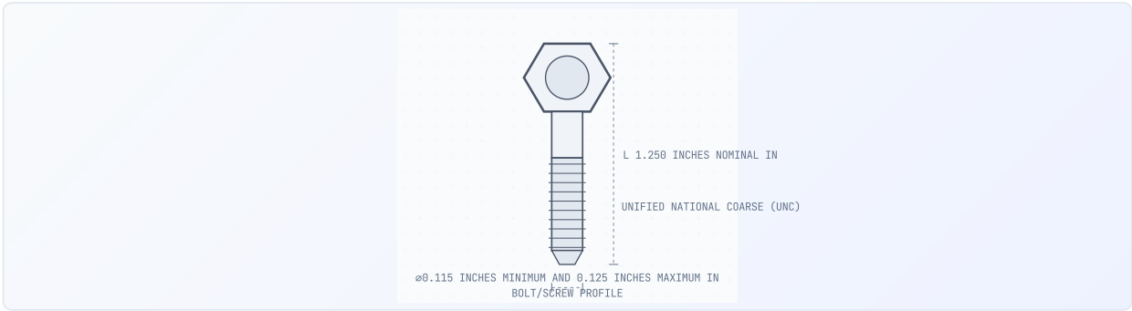
5305-01-059-7406 — SCREWS
