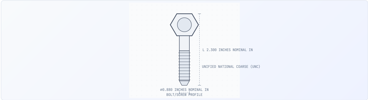
5305-01-059-0121 — SCREWS
