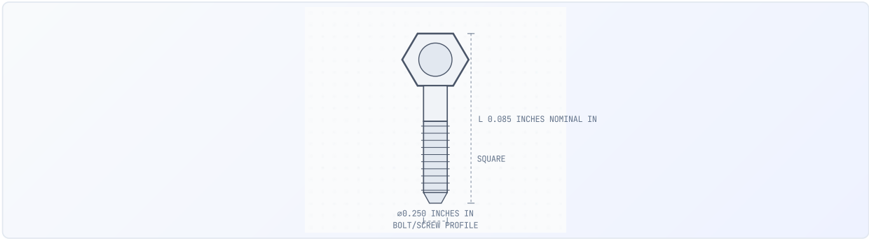
5305-00-162-5563 — SCREWS
